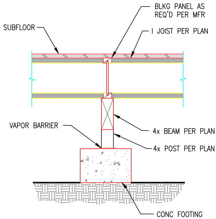
TS17 TYPICAL INTERMEDIATE BRG WITH POST
