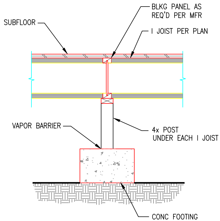
TS16 TYPICAL INTERMEDIATE BRG WITH POST
