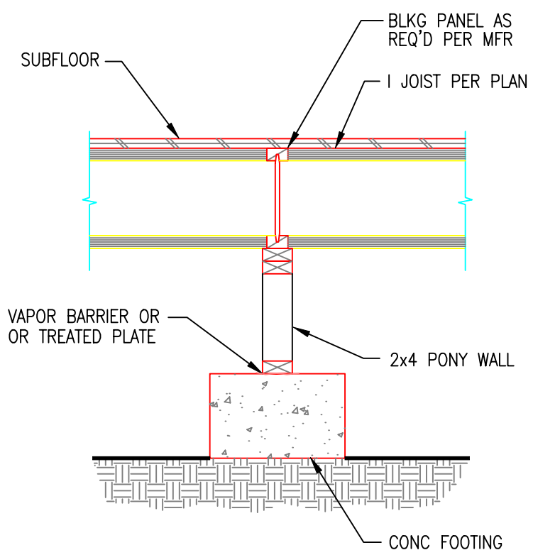
TS15 TYPICAL INTERMEDIATE BRG WITH PONY WALL SCALE: 3/4"=1'-0"
