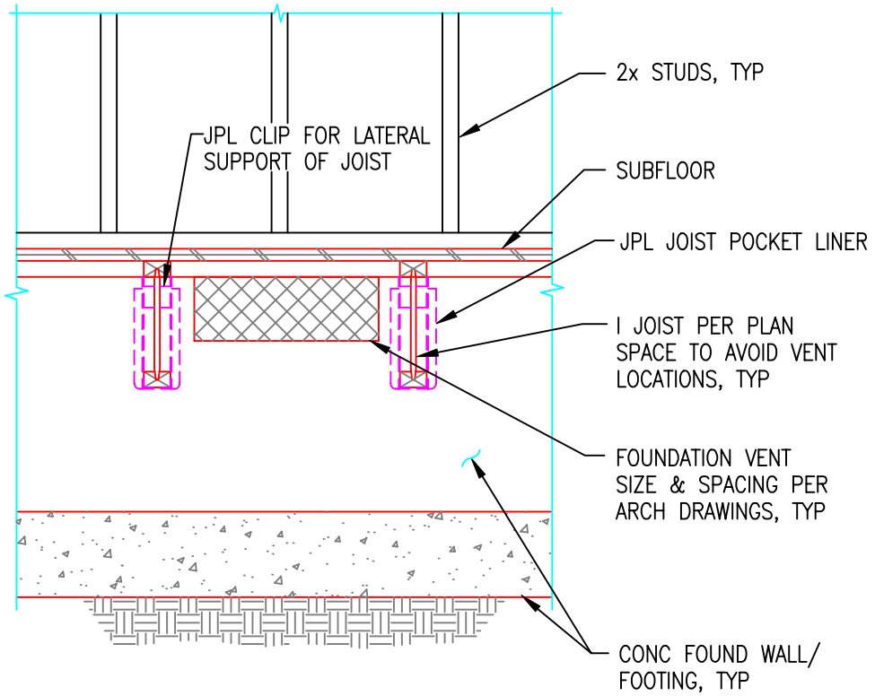
TS14 TYPICAL JPL JOIST POCKET LINER @ VENT SCALE: 3/4"=1'-0"
